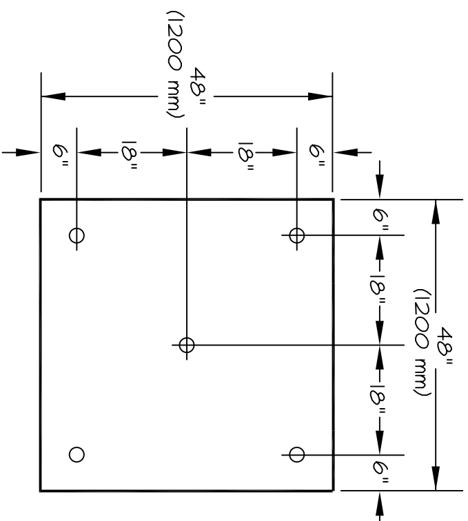
4' (1200 mm) x 4' (1200 mm) INSULATION BOARDS
