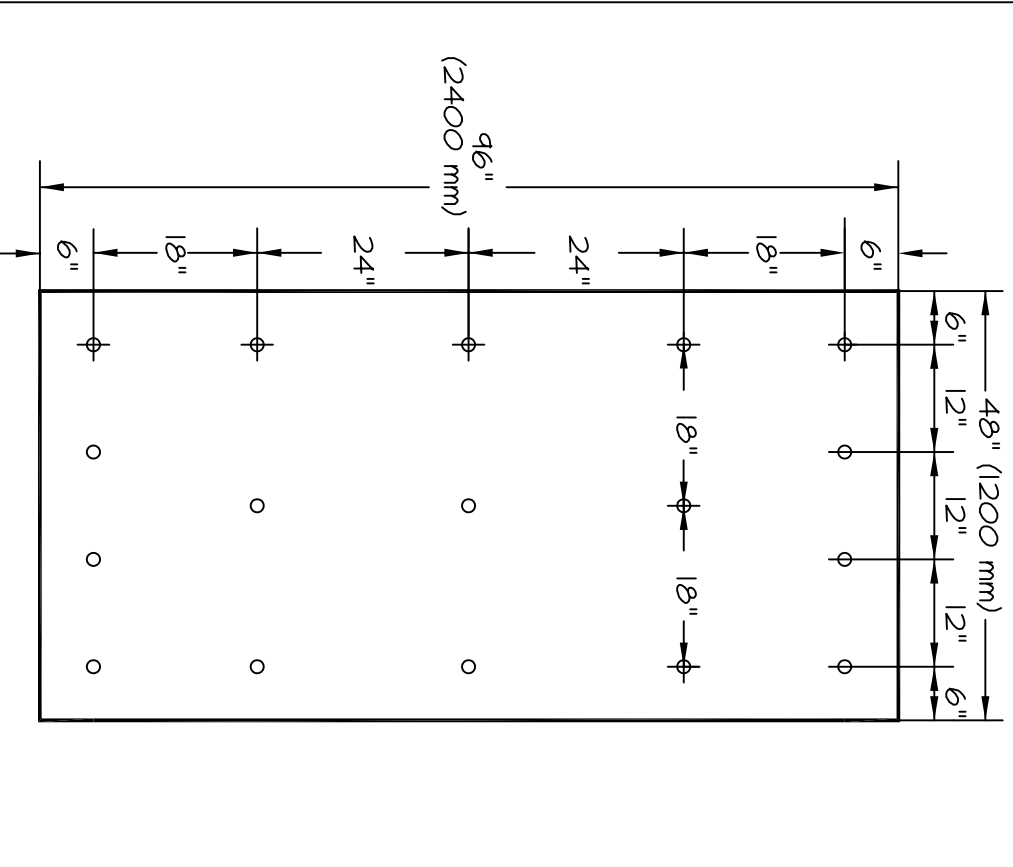
4' (1200 mm) X 8' (2400 mm) ORIENTED STRAND BOARD
